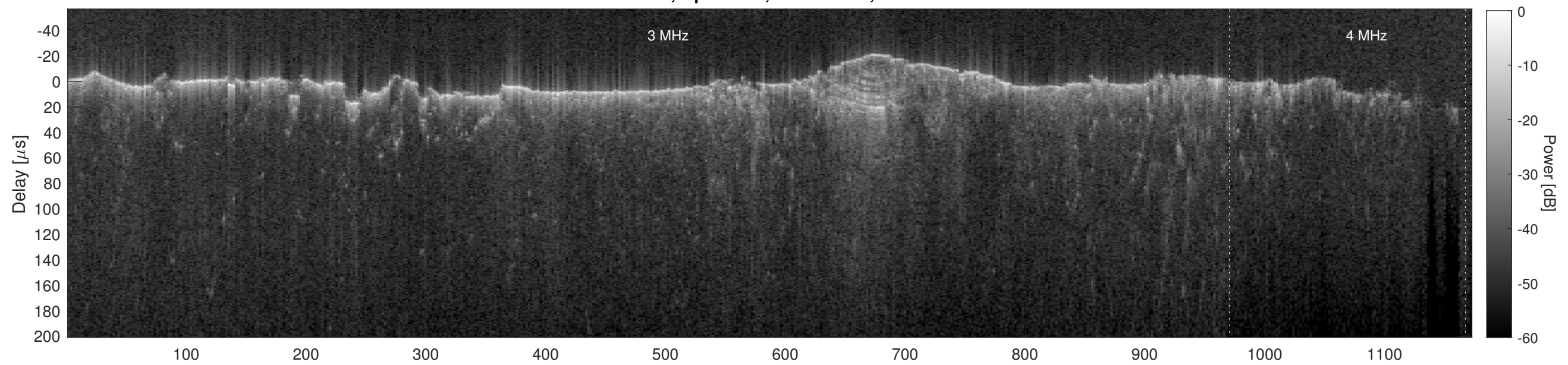
Orbit 12982, Cluttergram
