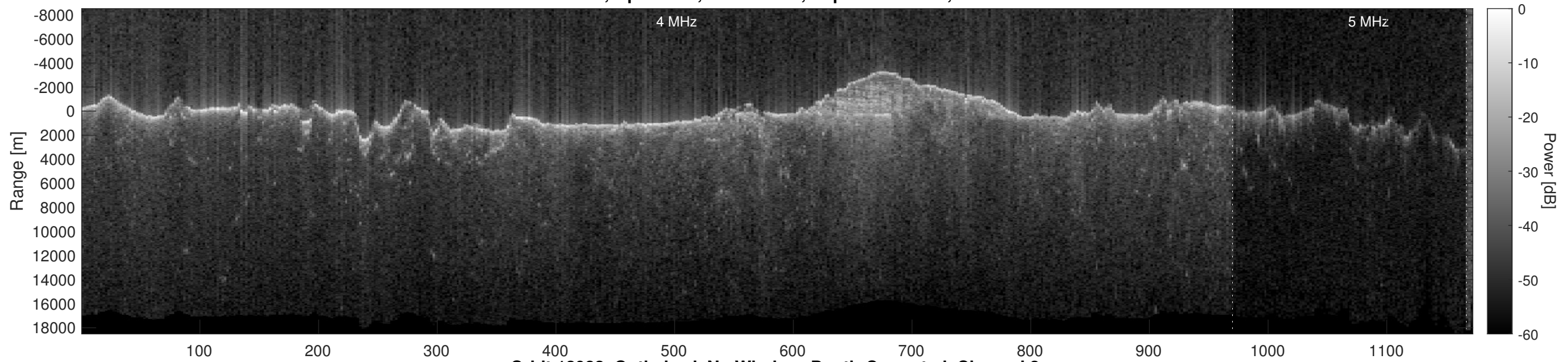
Orbit 12982, Optimized, No Window, Depth-Corrected, Channel 2
