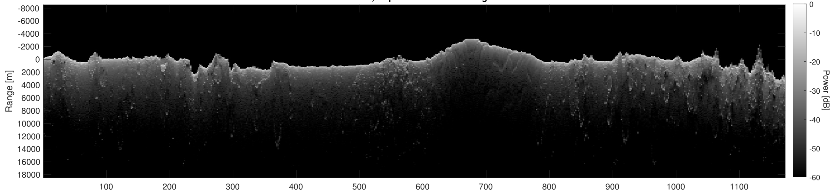
Orbit 12982, Depth-Corrected Cluttergram
