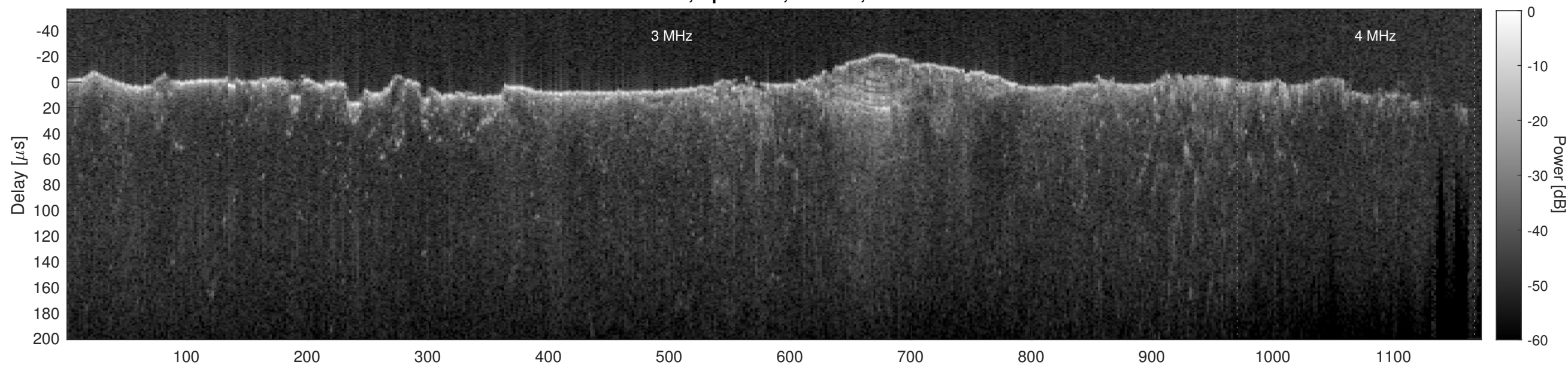
Orbit 12982, Cluttergram
