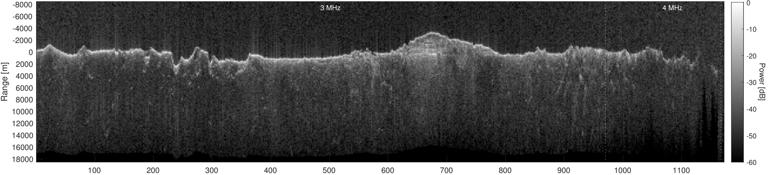
Orbit 12982, Depth-Corrected Cluttergram
