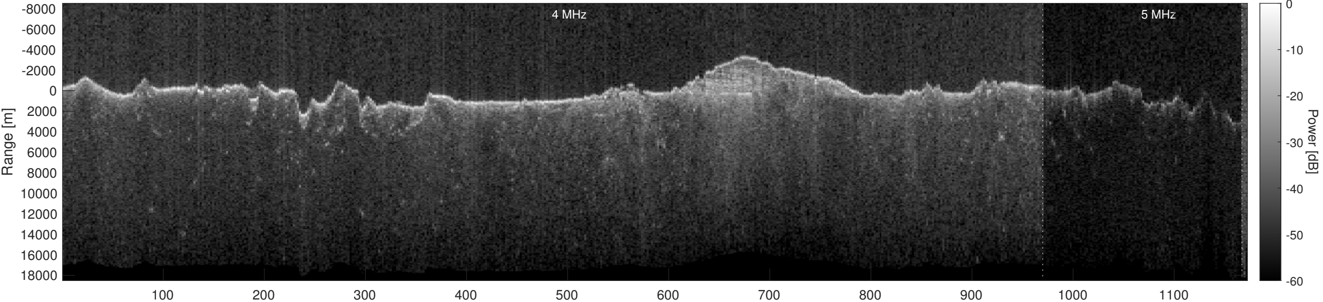
Orbit 12982, Optimized, Window, Depth-Corrected, Channel 2
