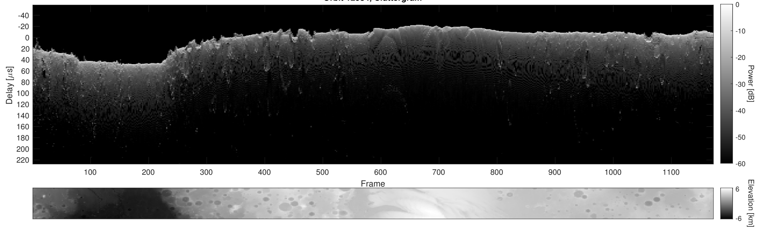
Orbit 12984, Cluttergram
