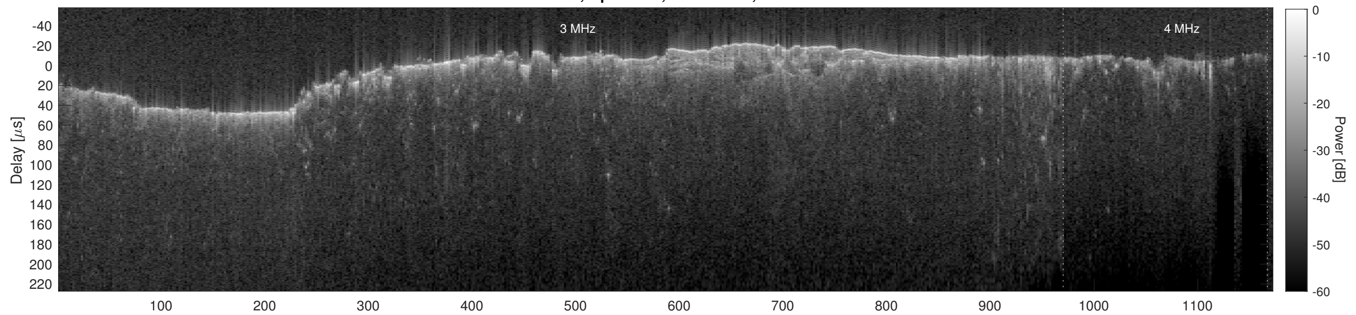
Orbit 12984, Cluttergram
