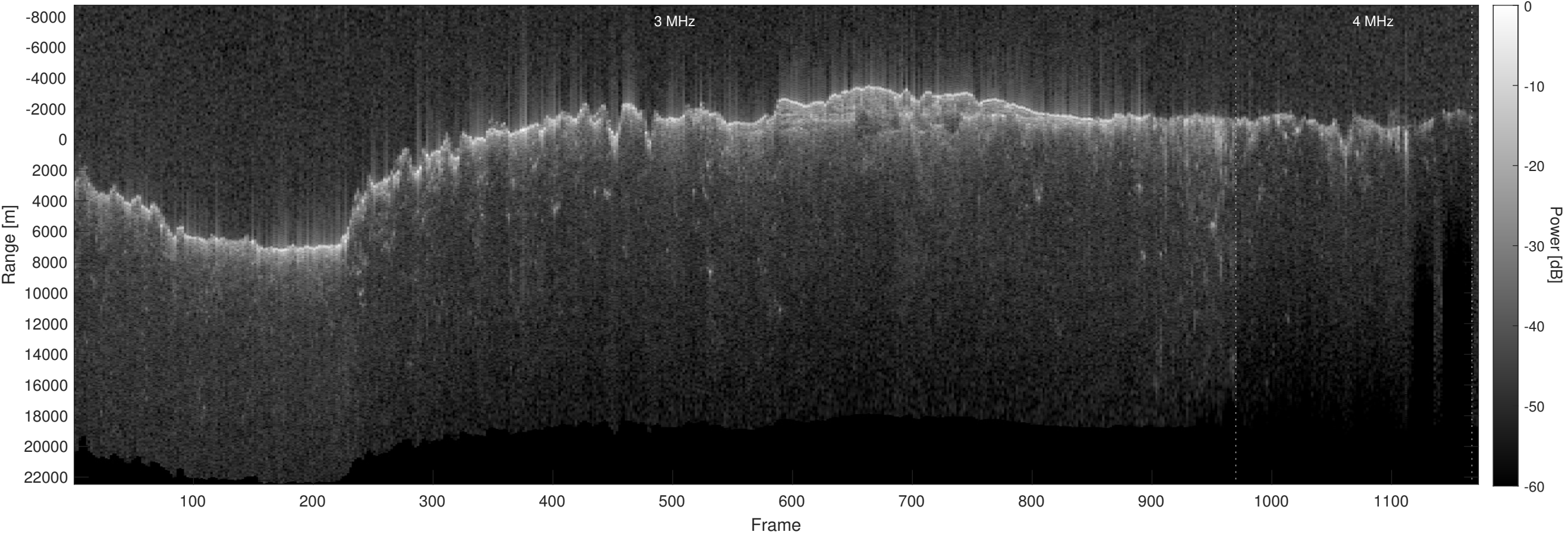
Orbit 12984, Optimized, No Window, Depth-Corrected, Channel 2
