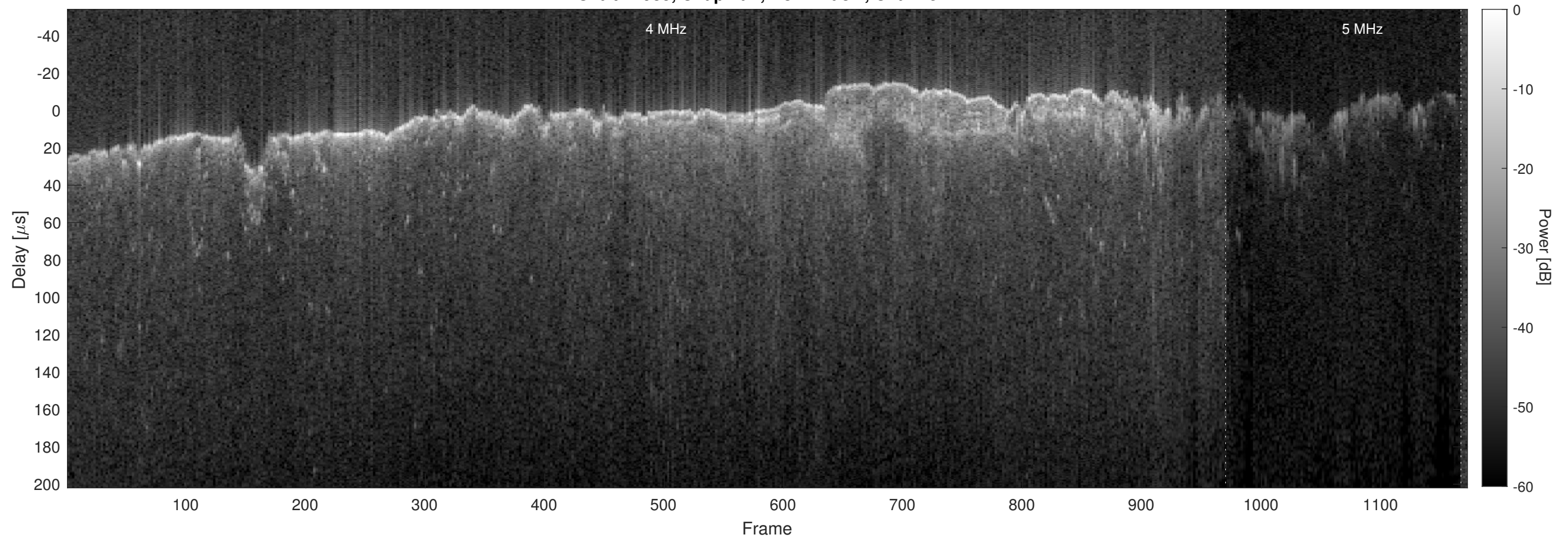
Orbit 12985, Chapman, No Window, Channel 2
