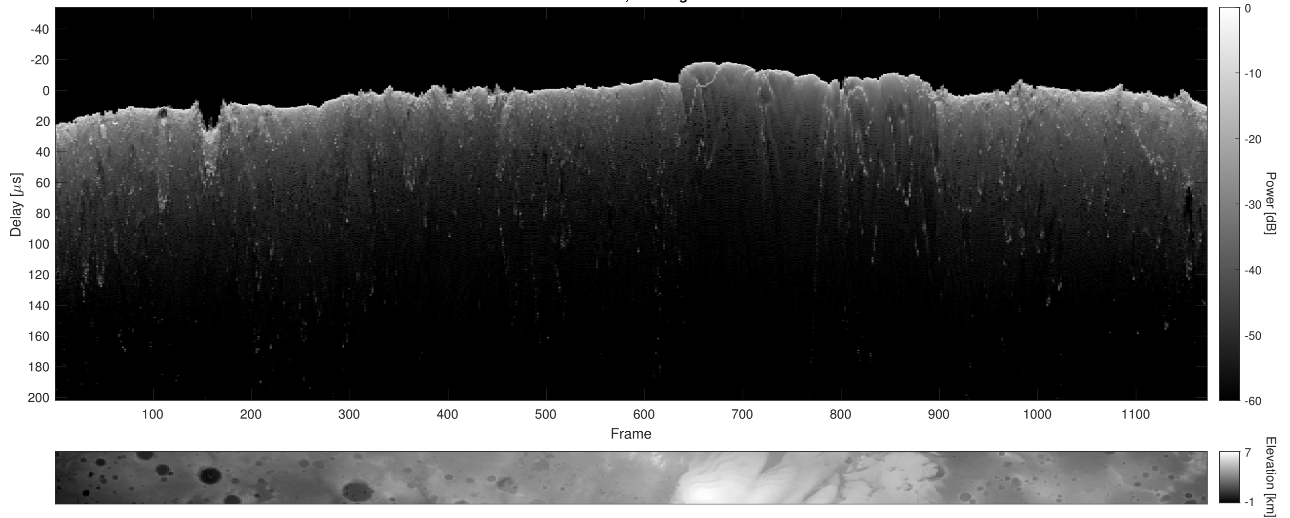
Orbit 12985, Cluttergram
