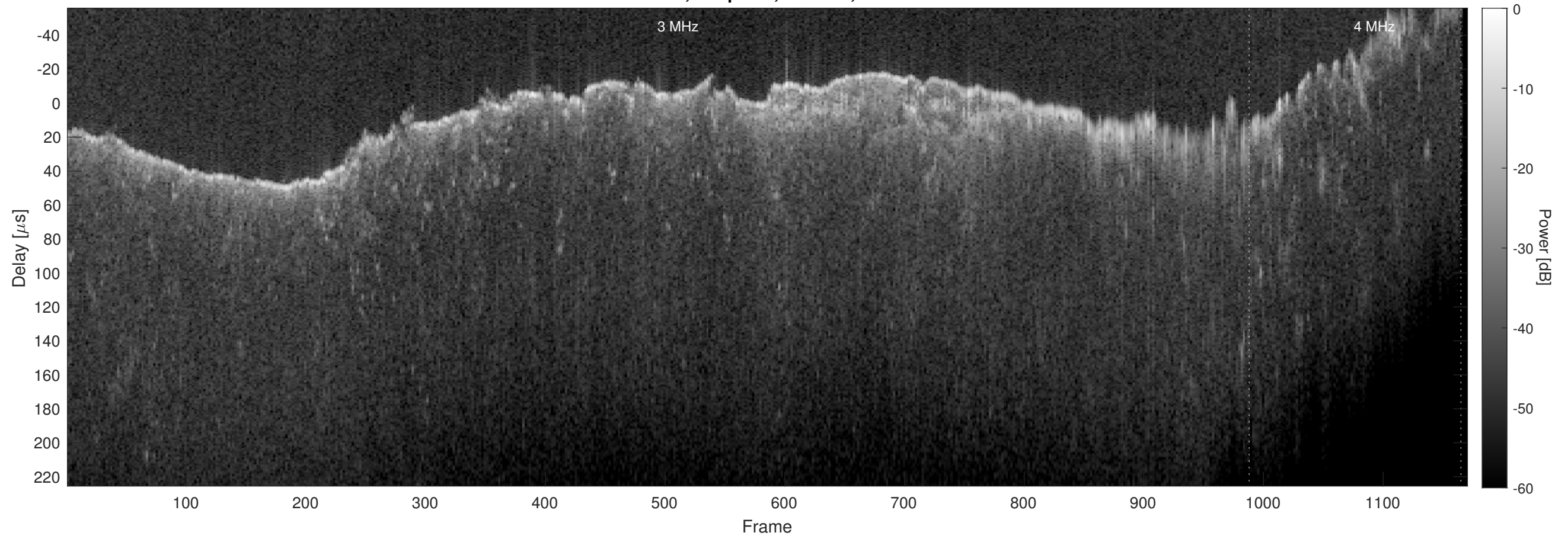
Orbit 12991, Chapman, Window, Channel 2
