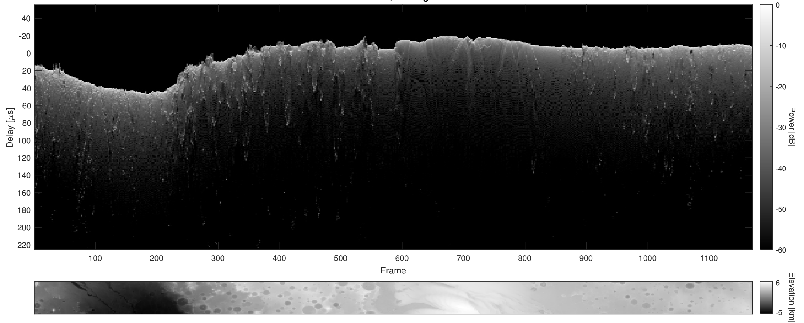
Orbit 12991, Cluttergram
