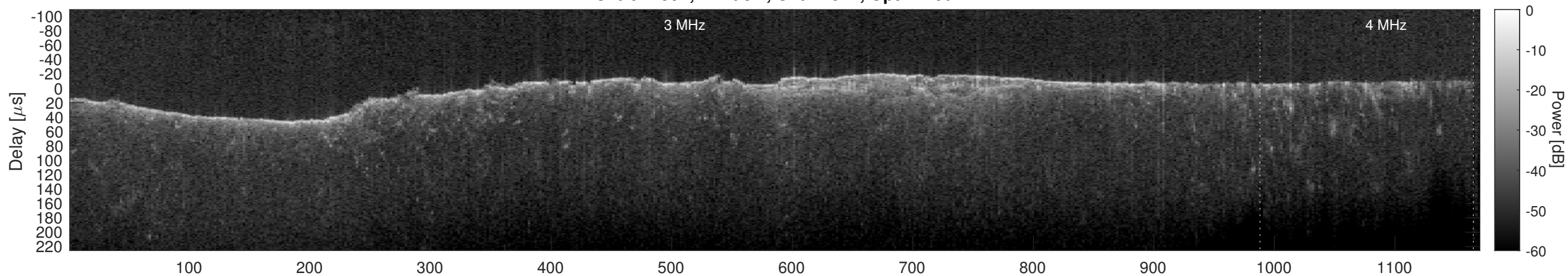
Orbit 12991, Cluttergram
