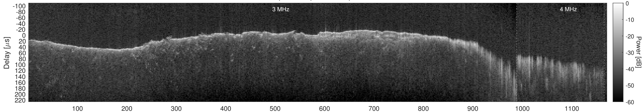
Orbit 12991, Window, Channel 2, Chapman
