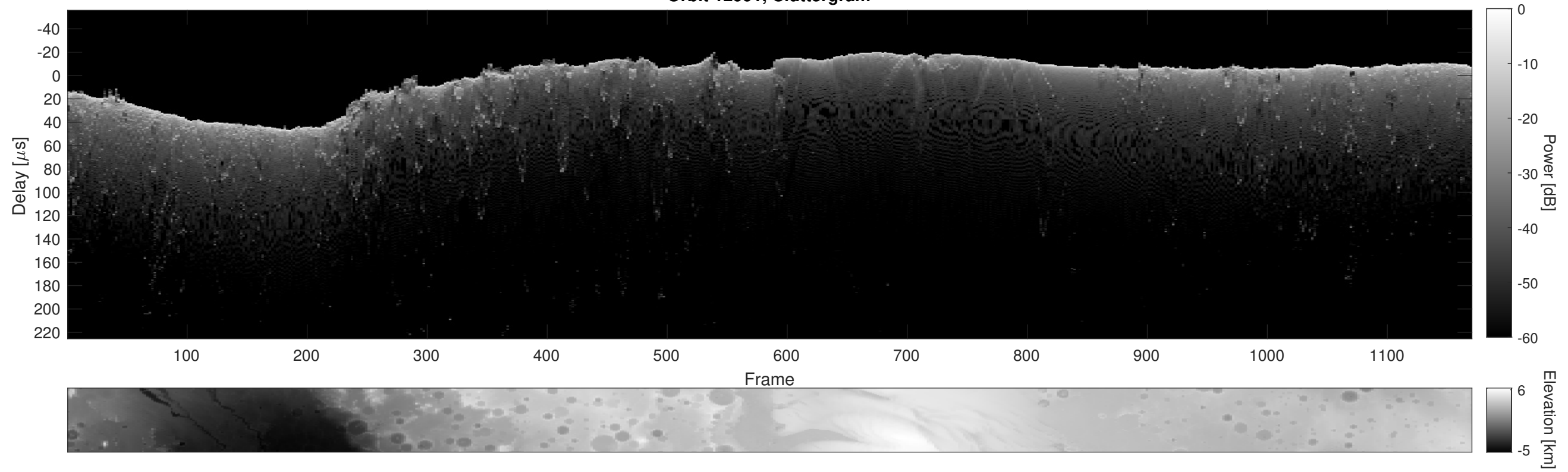
Orbit 12991, Cluttergram
