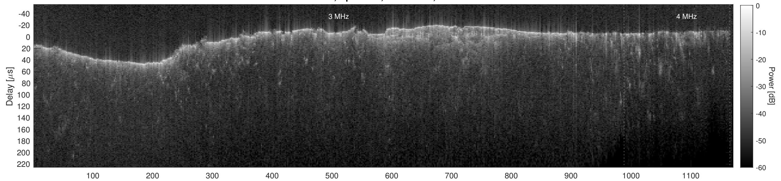
Orbit 12991, Cluttergram
