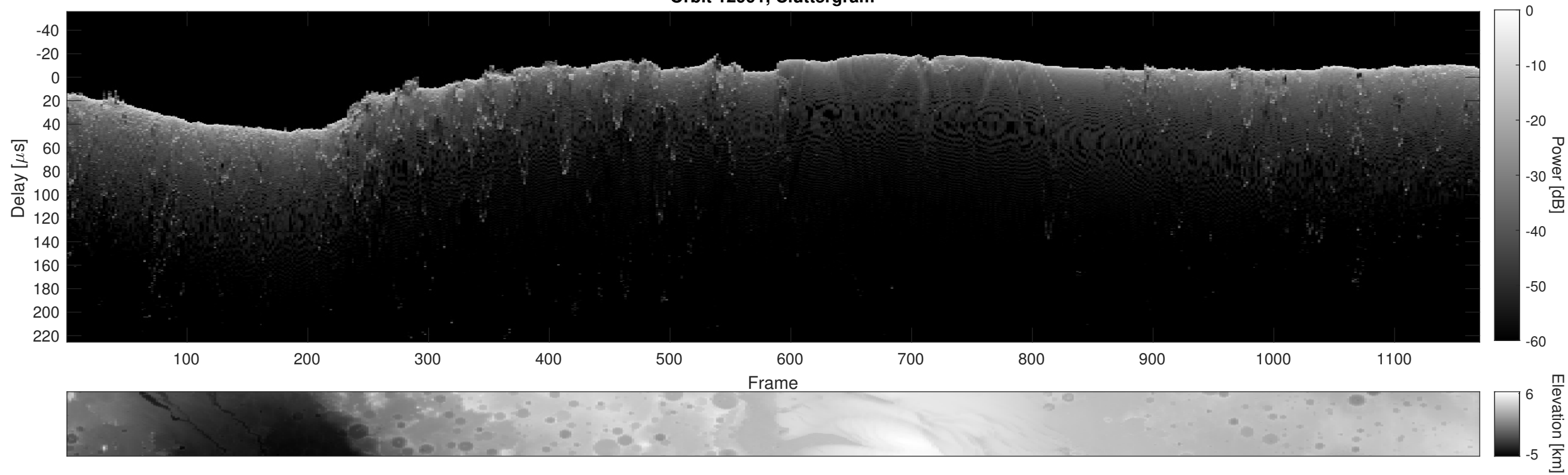
Orbit 12991, Cluttergram
