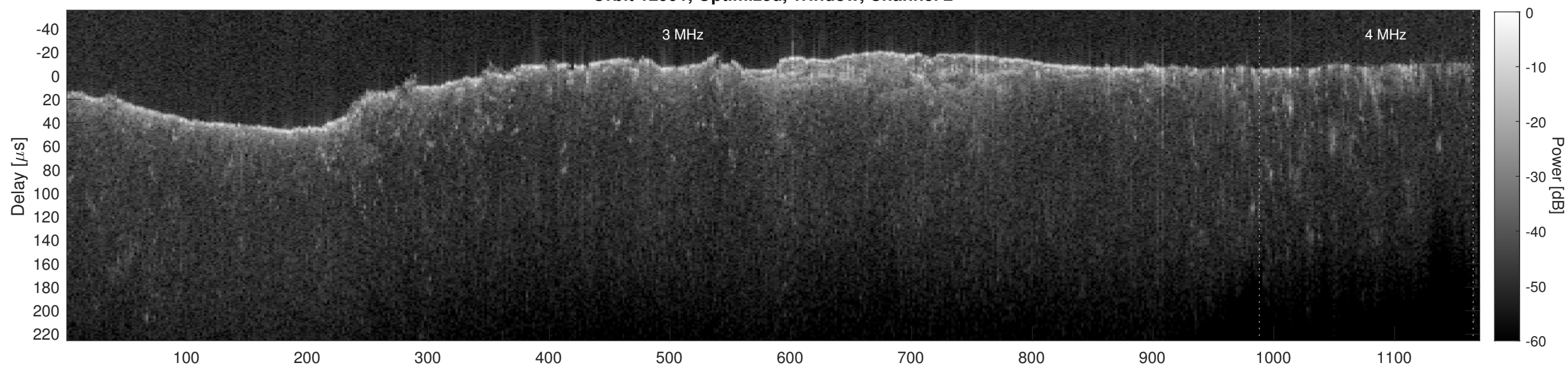
Orbit 12991, Cluttergram
