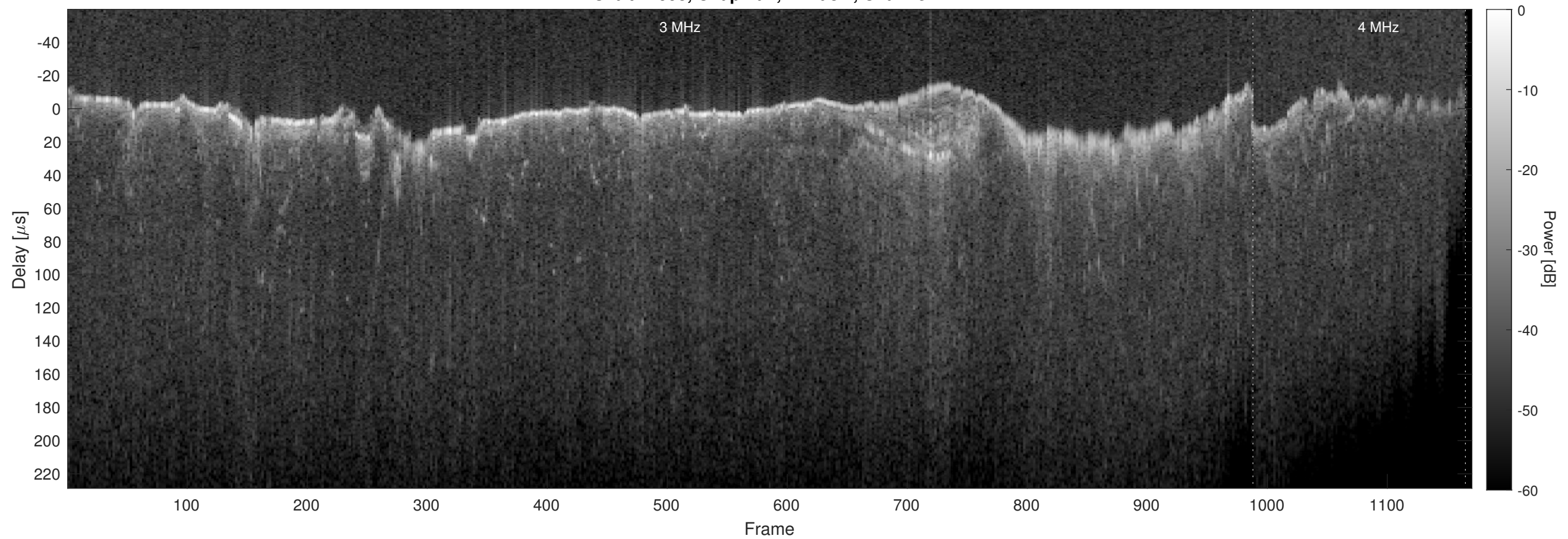
Orbit 12993, Chapman, Window, Channel 2
