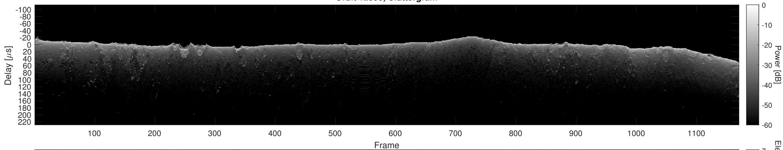
Orbit 12993, Cluttergram
