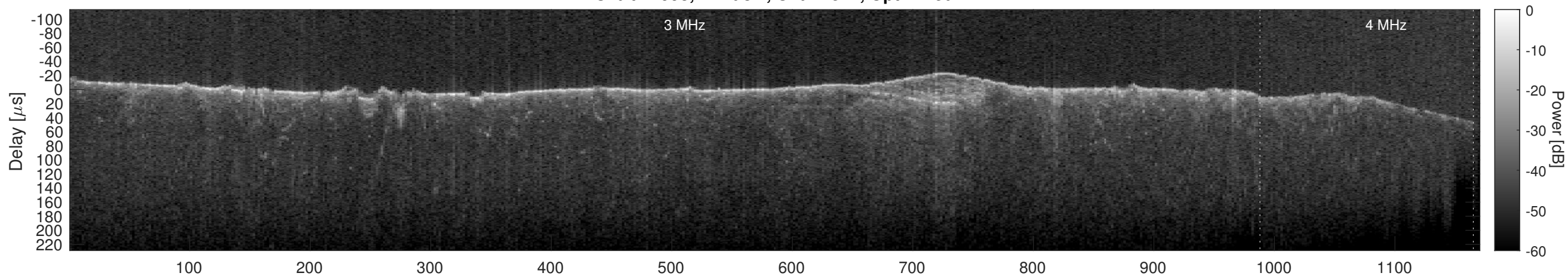
Orbit 12993, Cluttergram
