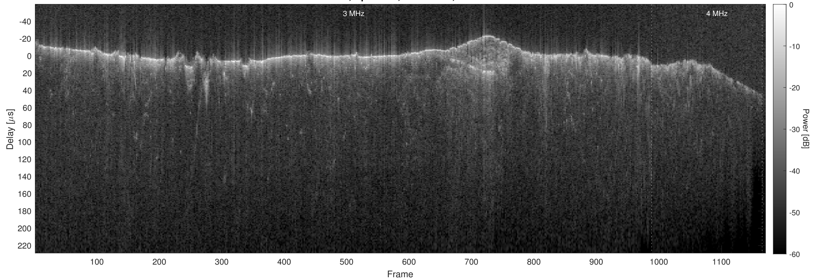
Orbit 12993, Optimized, No Window, Channel 2
