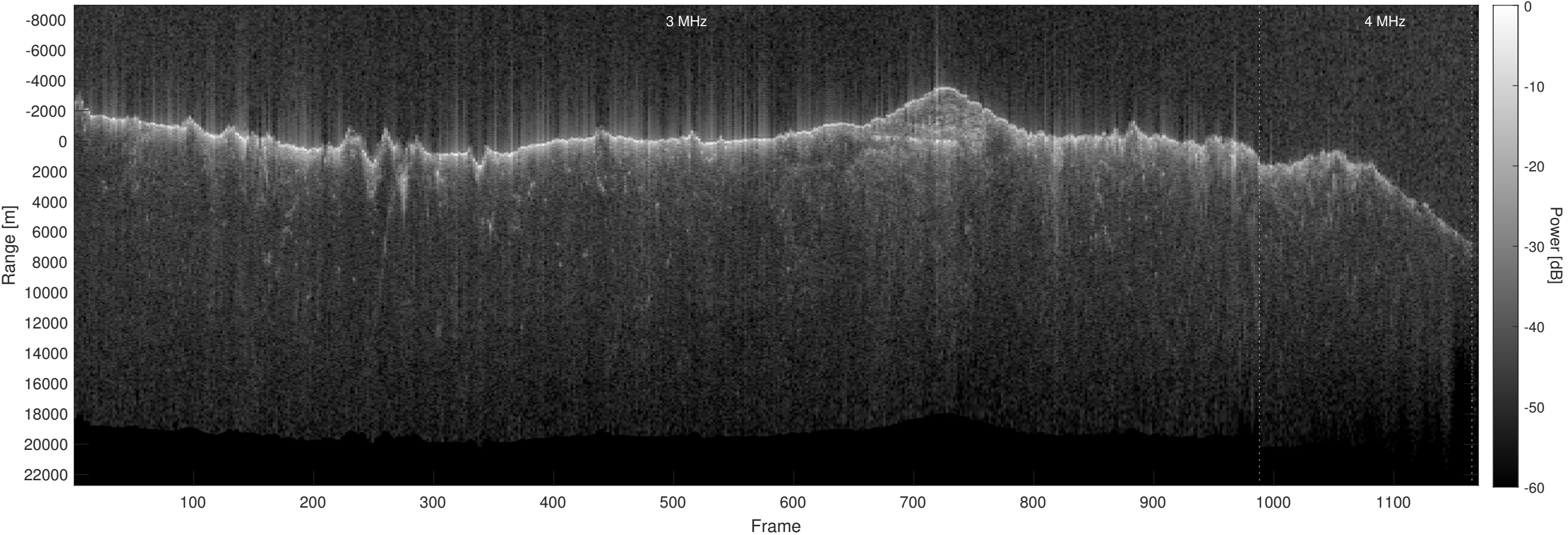
Orbit 12993, Optimized, No Window, Depth-Corrected, Channel 2
