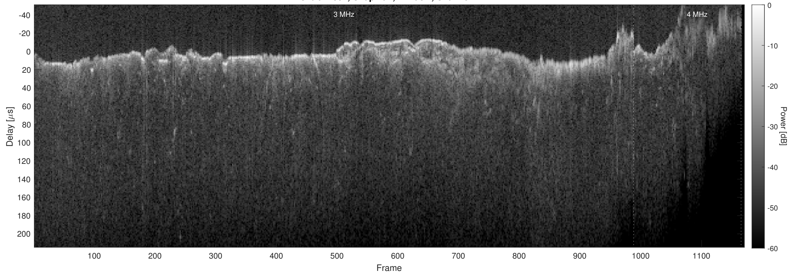
Orbit 12994, Chapman, Window, Channel 2
