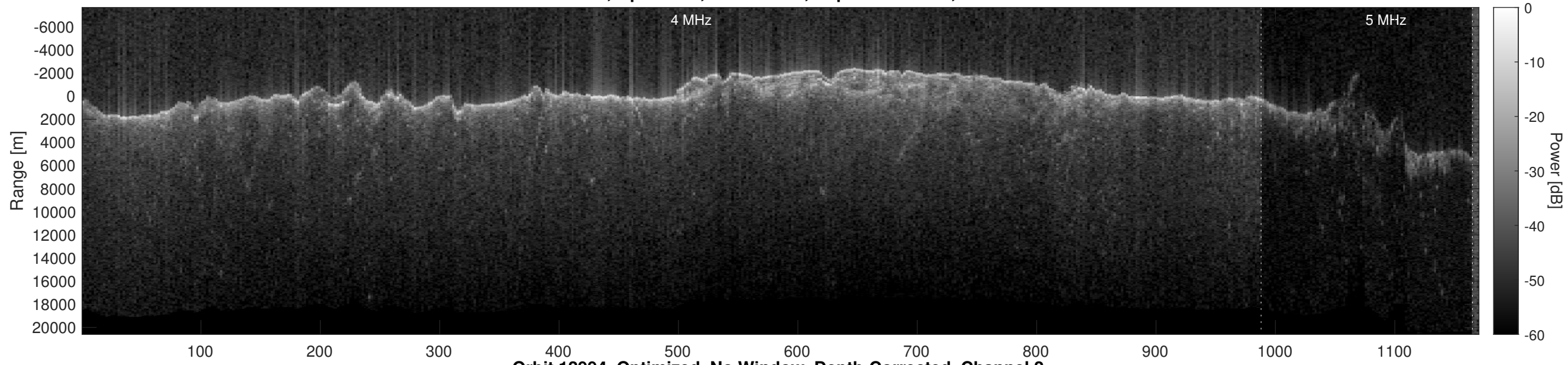
Orbit 12994, Optimized, No Window, Depth-Corrected, Channel 2
