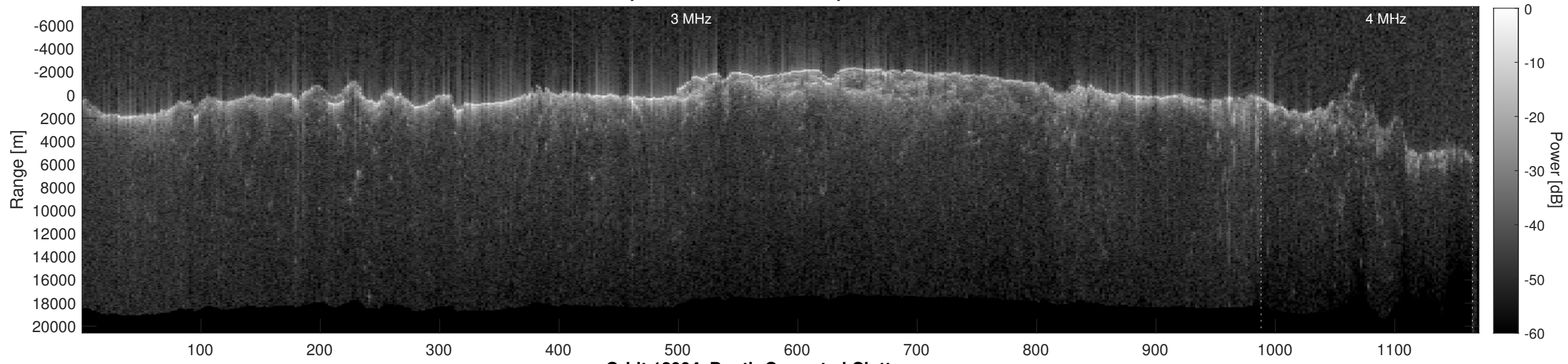
Orbit 12994, Depth-Corrected Cluttergram
