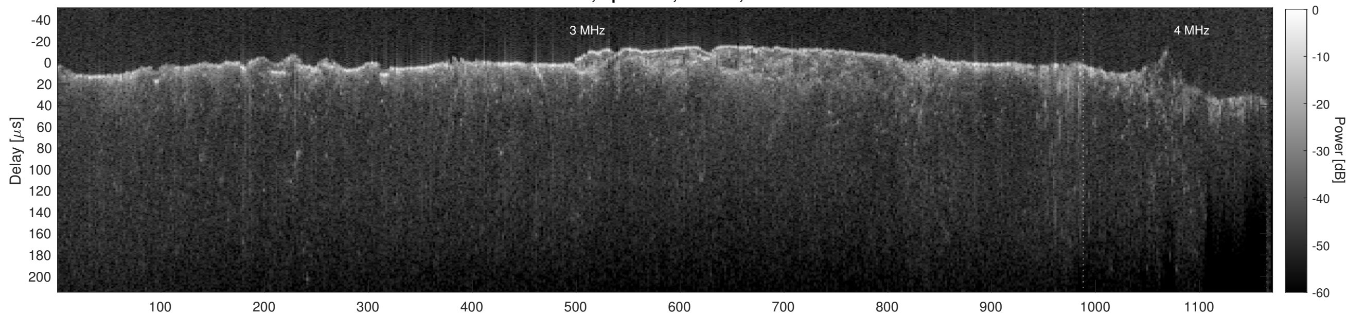
Orbit 12994, Cluttergram
