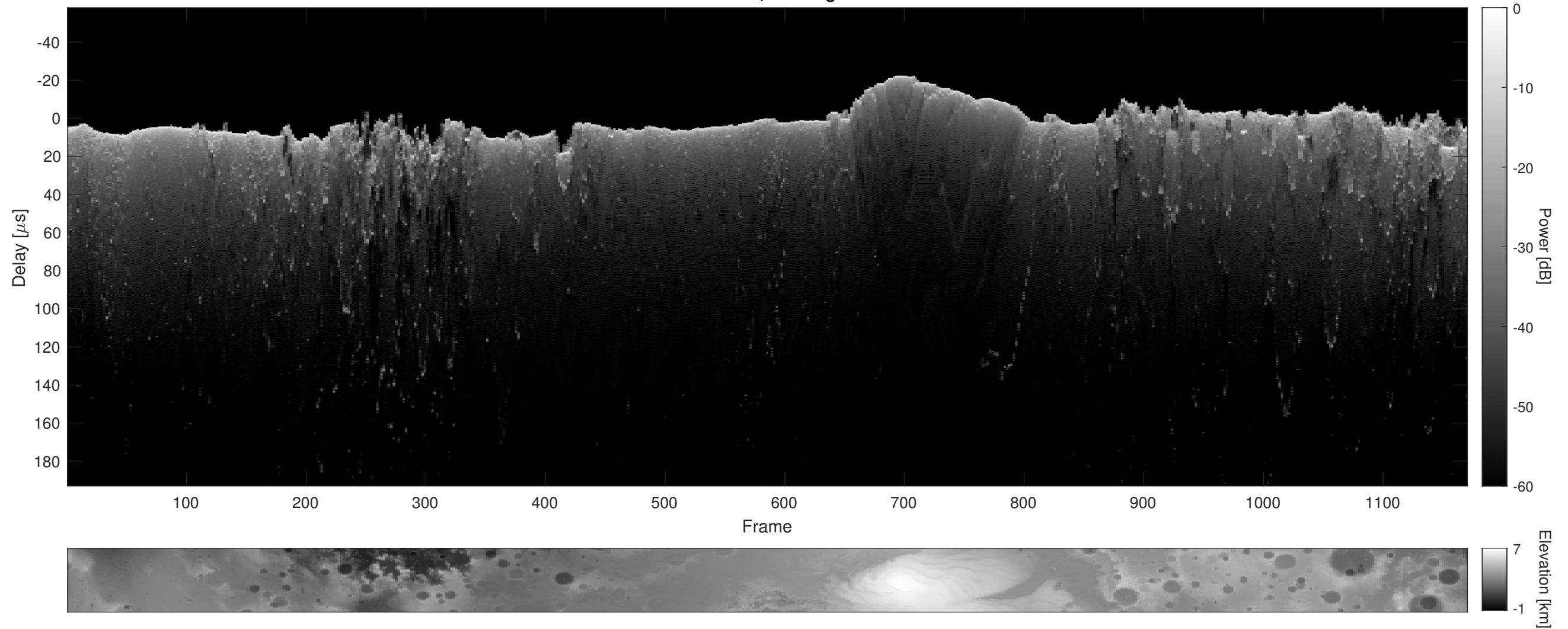
Orbit 12996, Cluttergram
