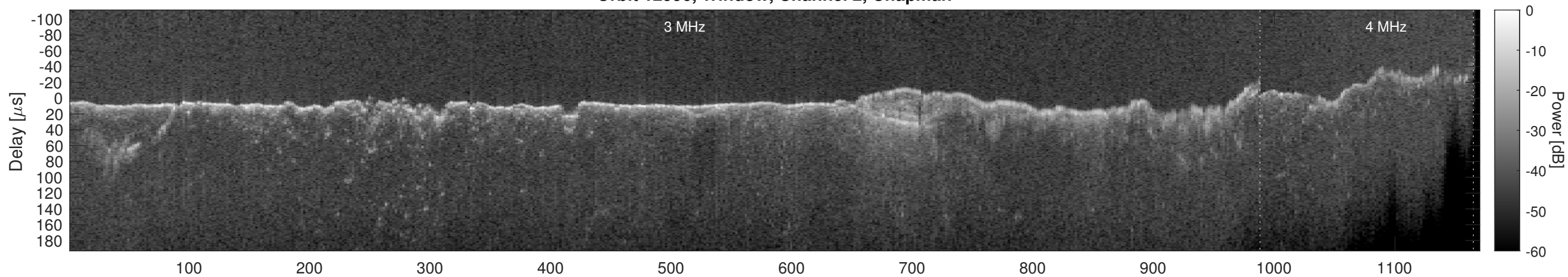
Orbit 12996, Window, Channel 2, Optimized
