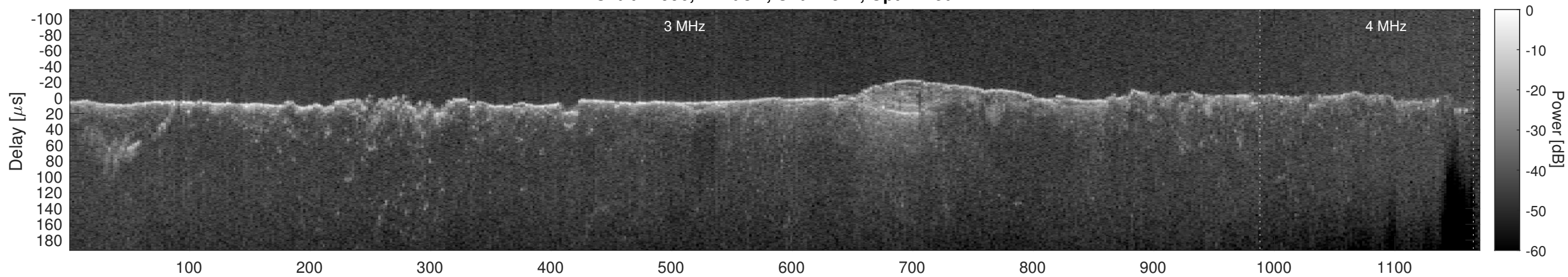
Orbit 12996, Cluttergram
