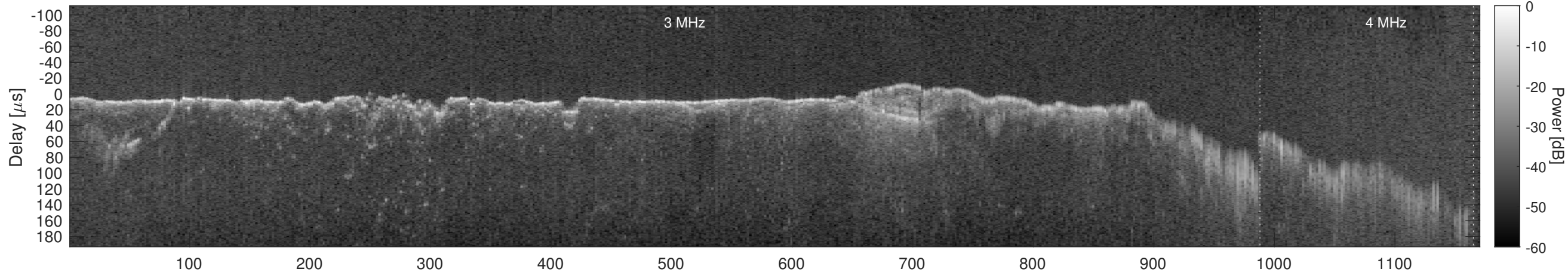
Orbit 12996, Window, Channel 2, Chapman
