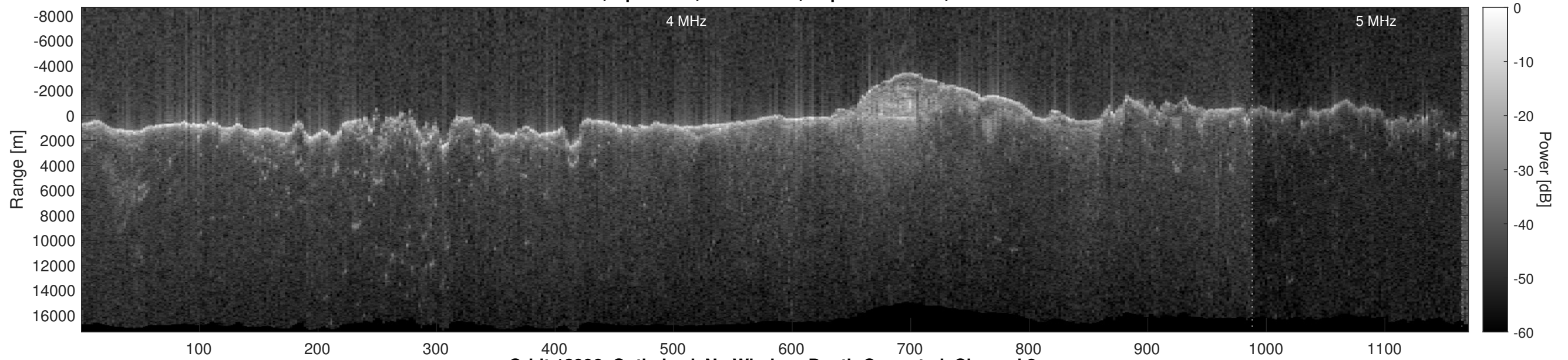
Orbit 12996, Optimized, No Window, Depth-Corrected, Channel 2
