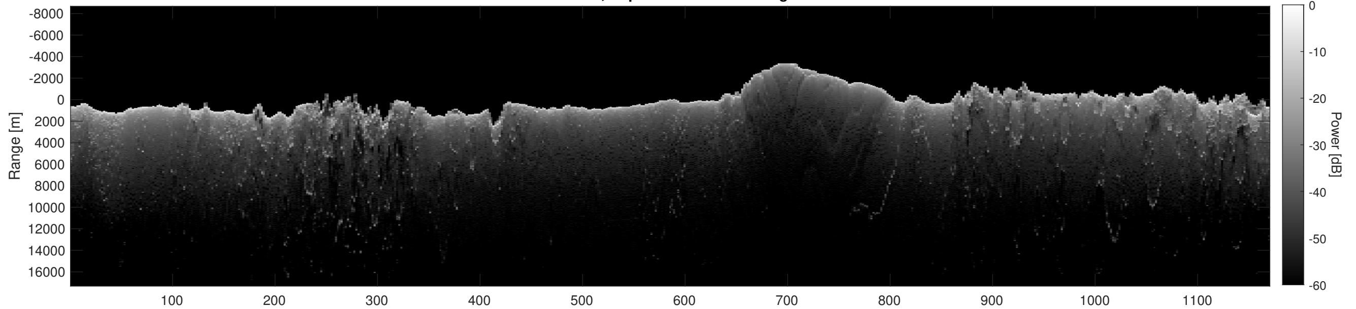
Orbit 12996, Depth-Corrected Cluttergram
