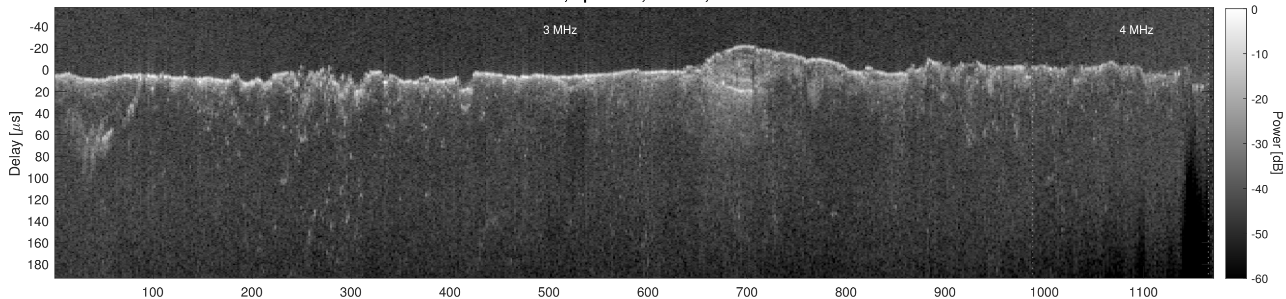
Orbit 12996, Cluttergram
