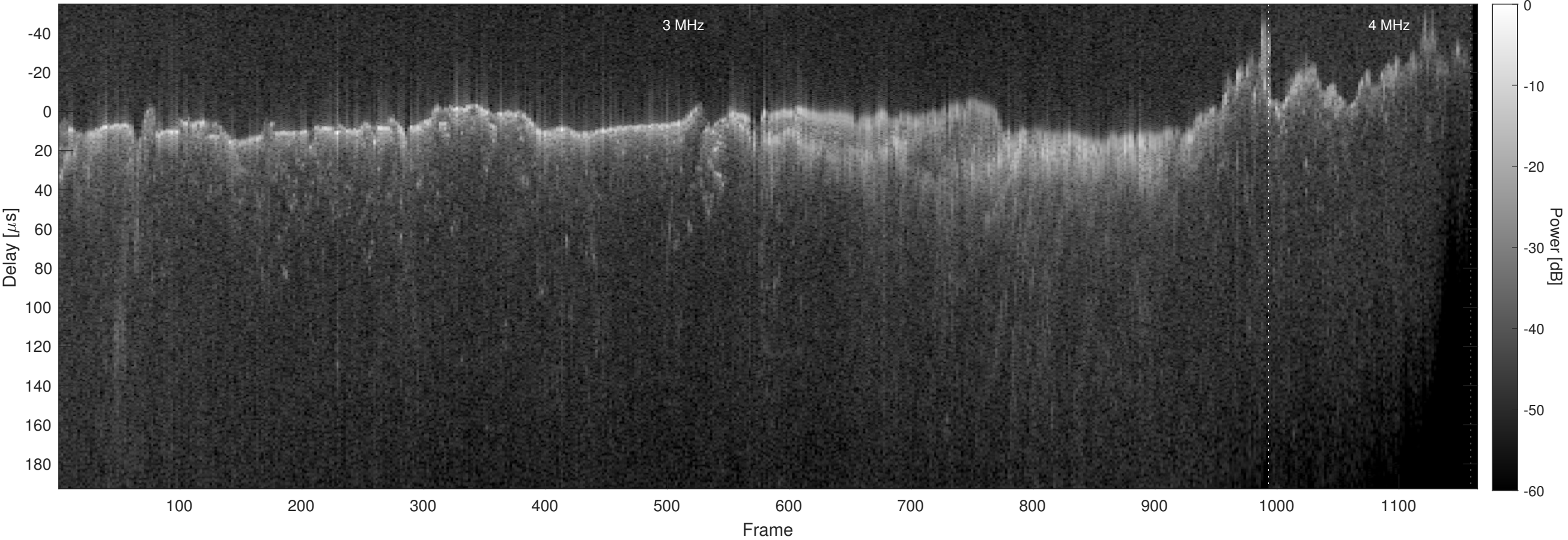
Orbit 12997, Chapman, No Window, Channel 2
