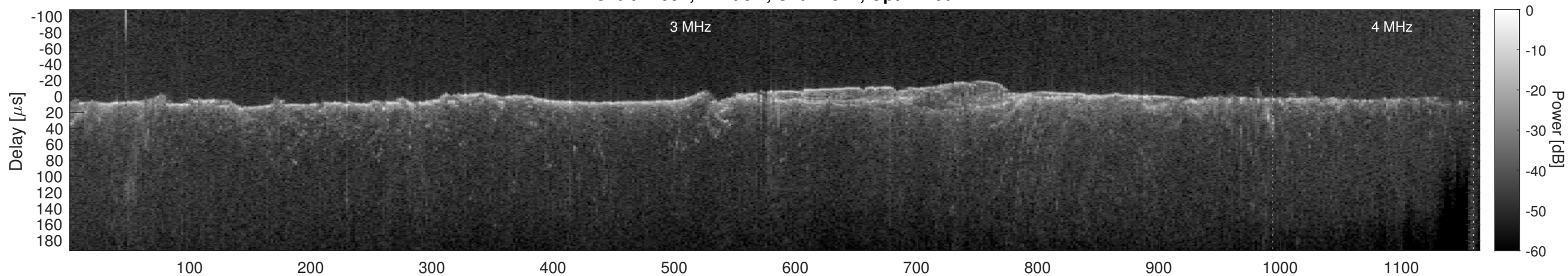
Orbit 12997, Cluttergram
