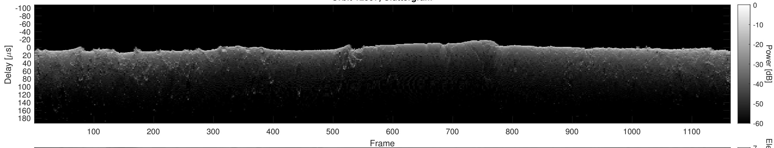
Orbit 12997, Cluttergram
