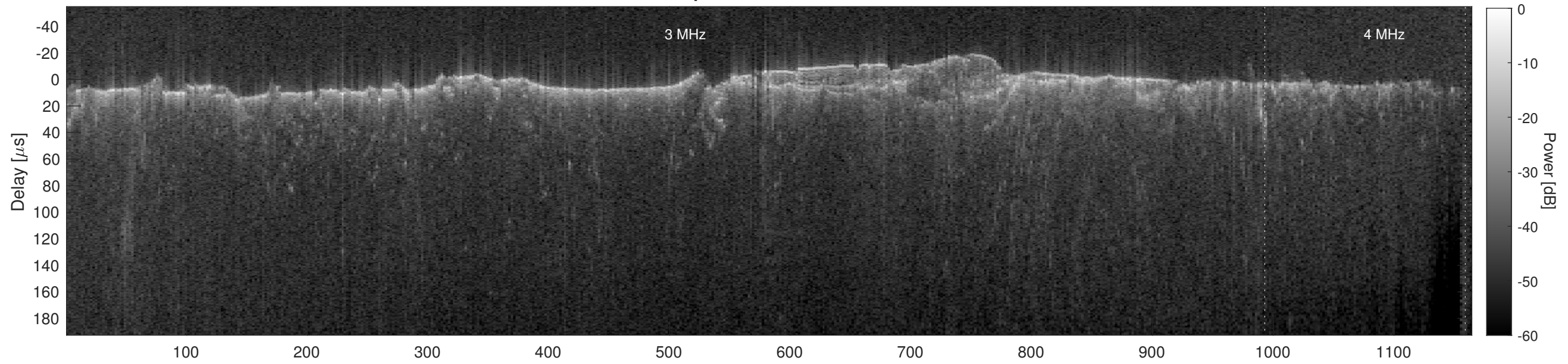
Orbit 12997, Cluttergram
