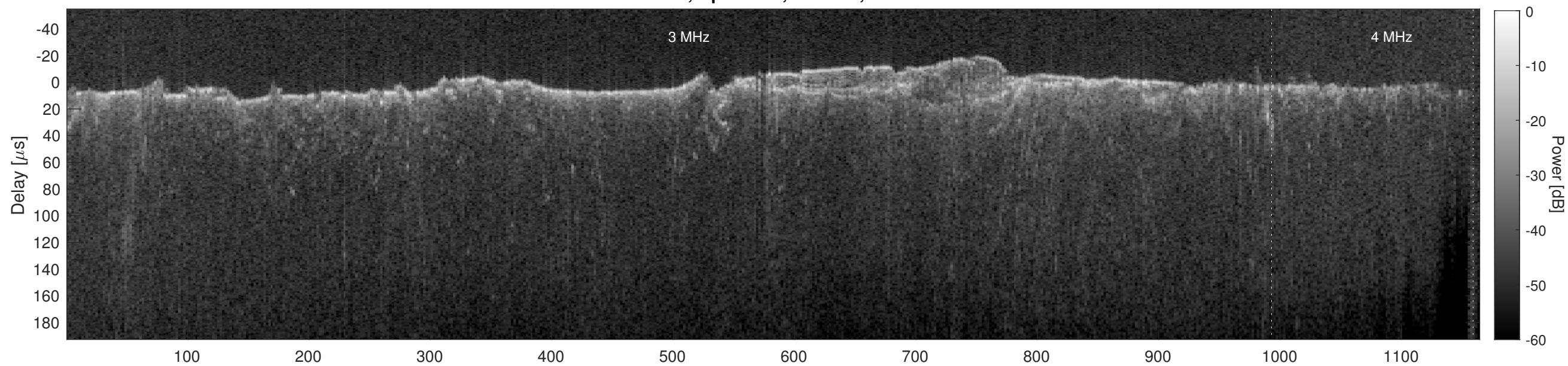
Orbit 12997, Cluttergram
