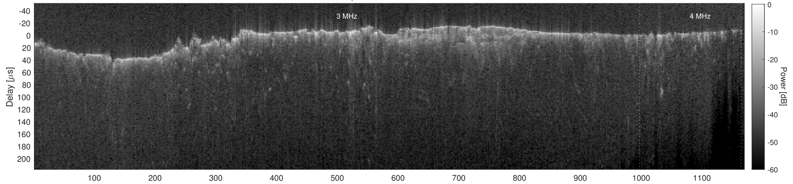
Orbit 12998, Cluttergram
