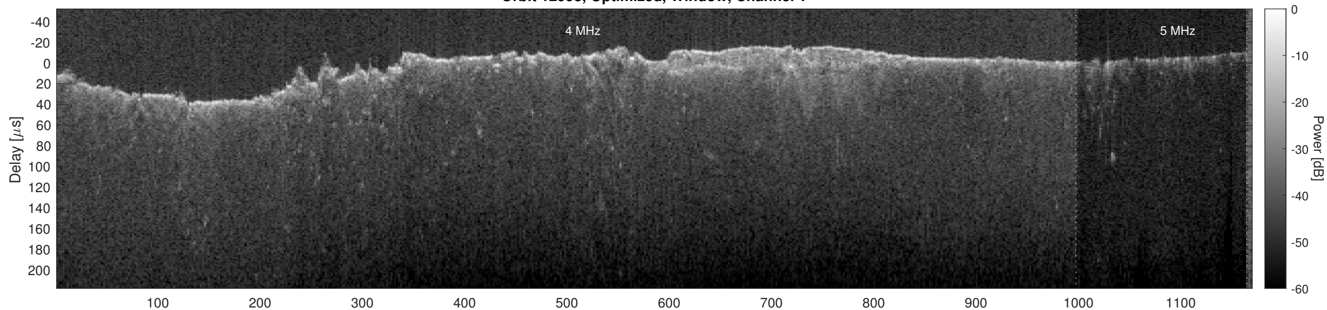
Orbit 12998, Optimized, Window, Channel 2
