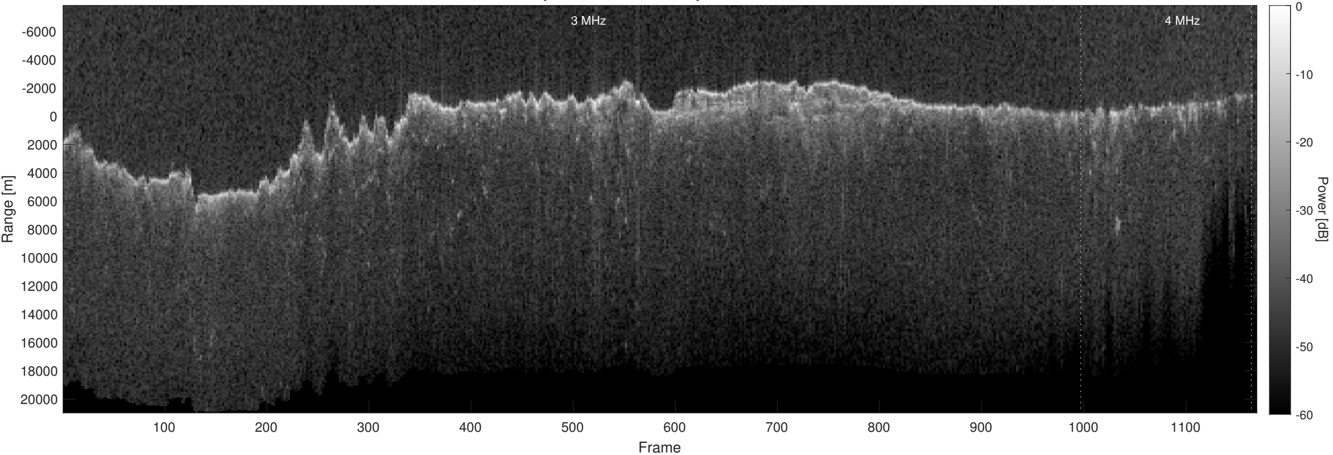
Orbit 12998, Optimized, Window, Depth-Corrected, Channel 2
