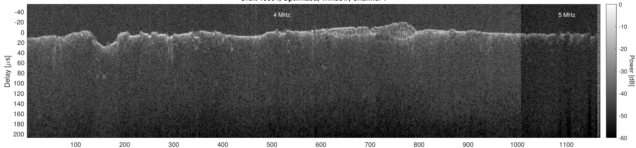
Orbit 13004, Optimized, Window, Channel 2
