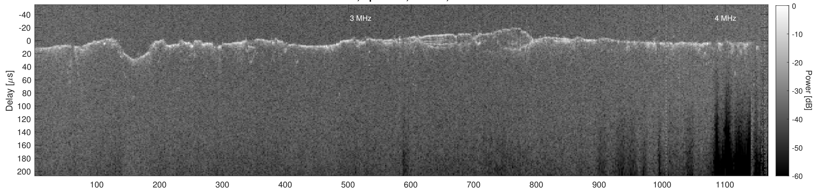
Orbit 13004, Cluttergram
