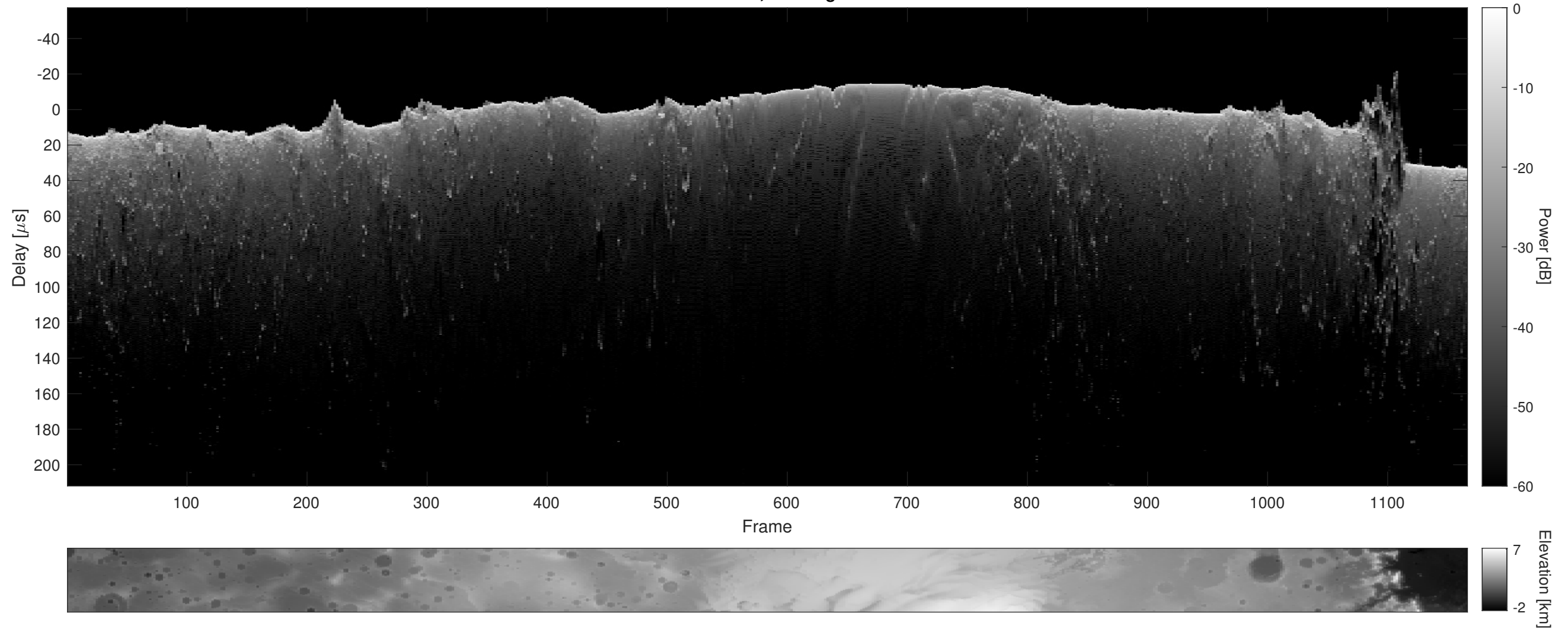
Orbit 13008, Cluttergram
