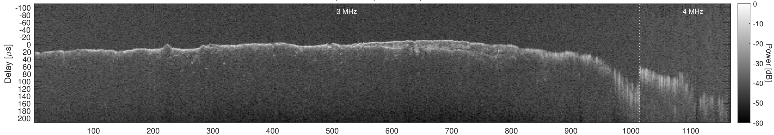
Orbit 13008, Window, Channel 2, Chapman
