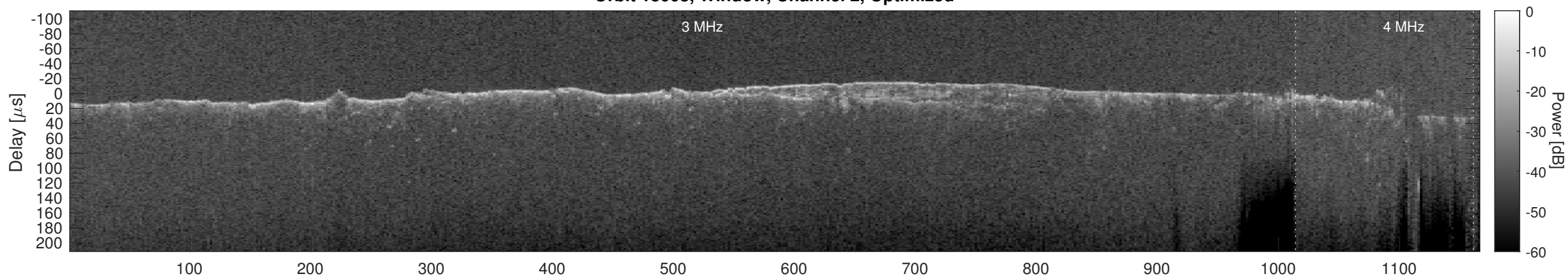
Orbit 13008, Cluttergram
