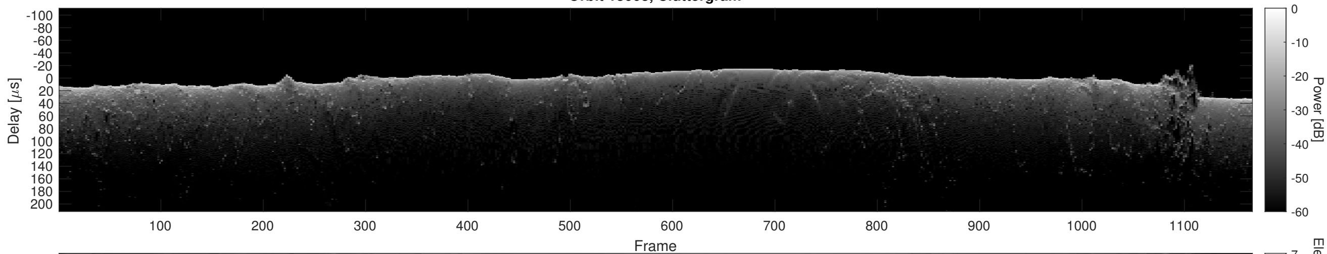
Orbit 13008, Cluttergram
