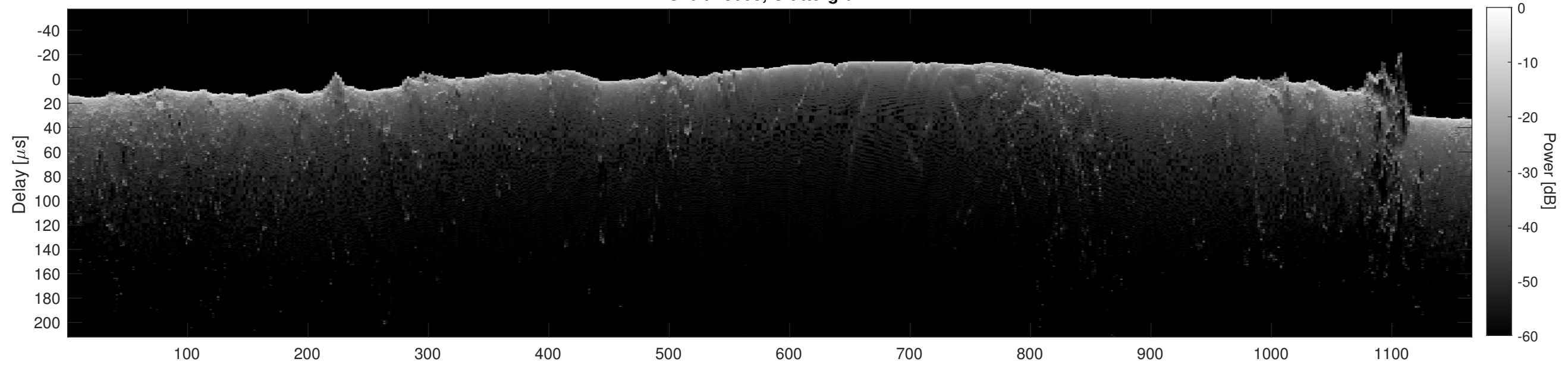
Orbit 13008, Cluttergram
