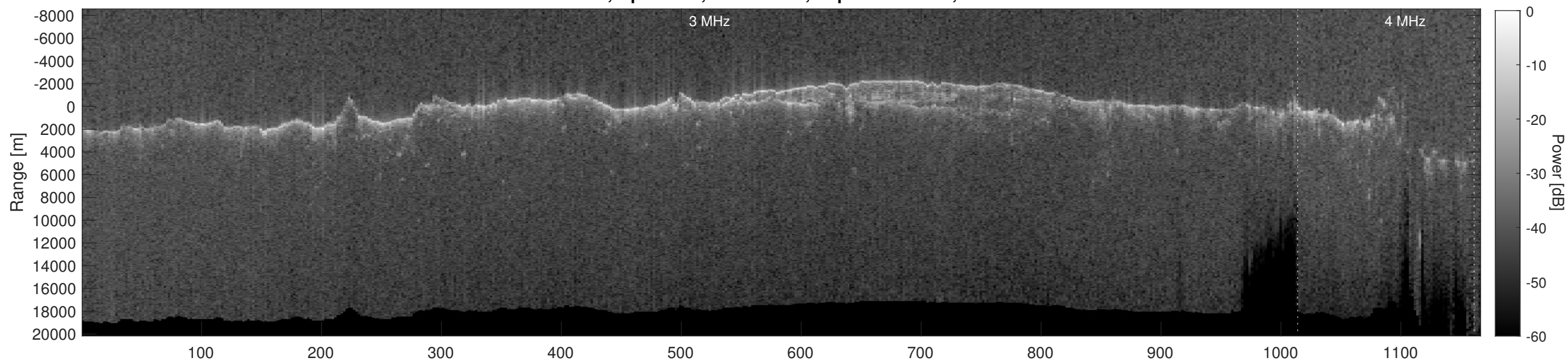
Orbit 13008, Depth-Corrected Cluttergram
