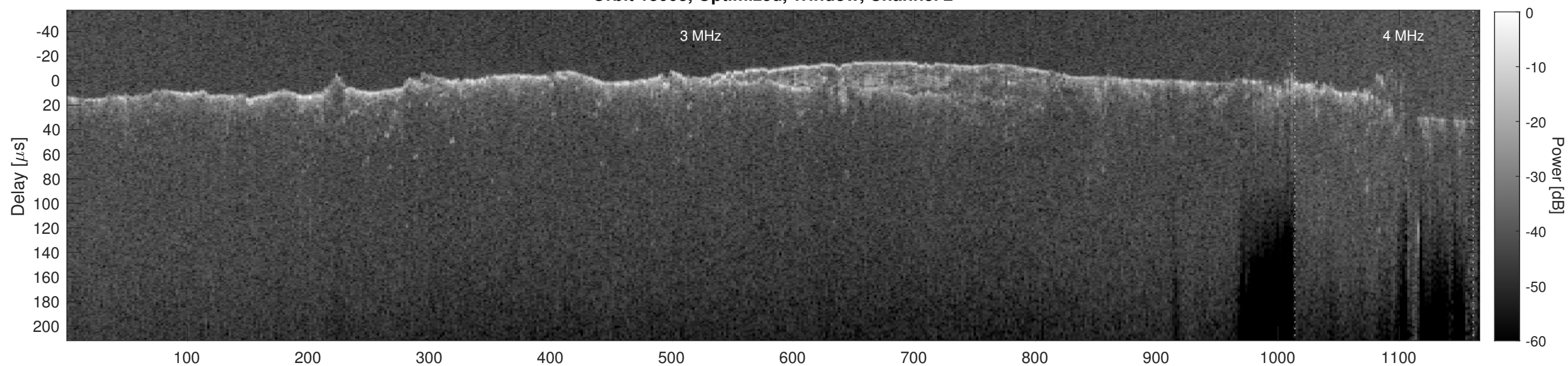
Orbit 13008, Cluttergram
