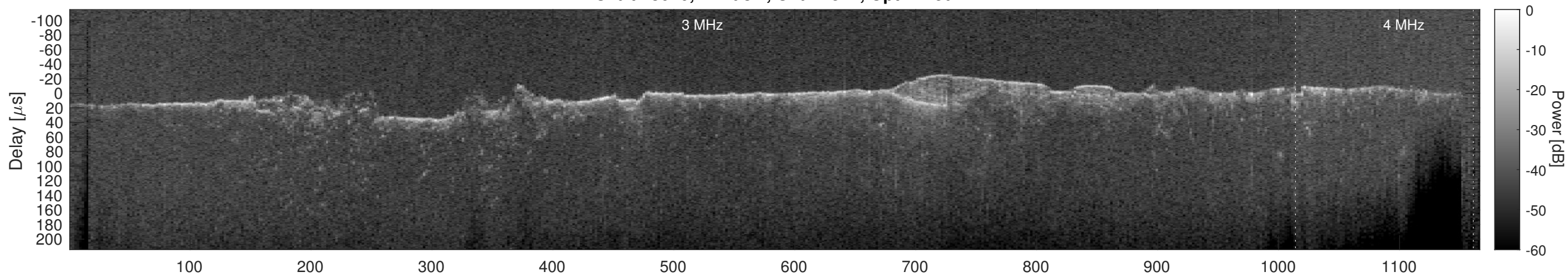
Orbit 13010, Cluttergram
