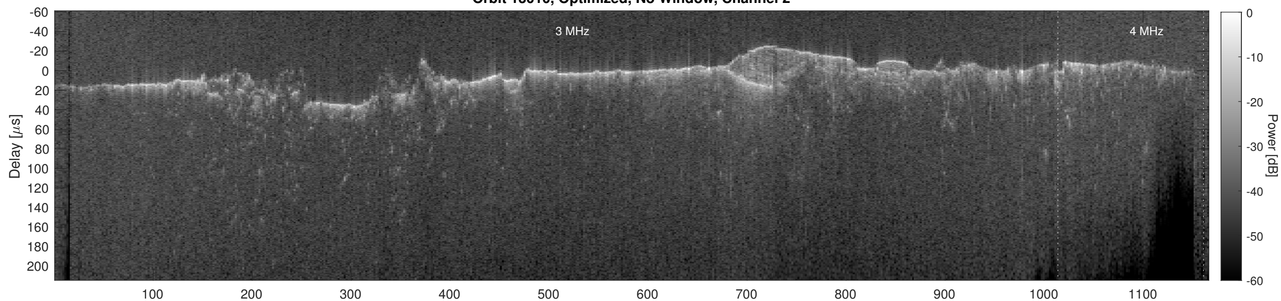
Orbit 13010, Cluttergram
