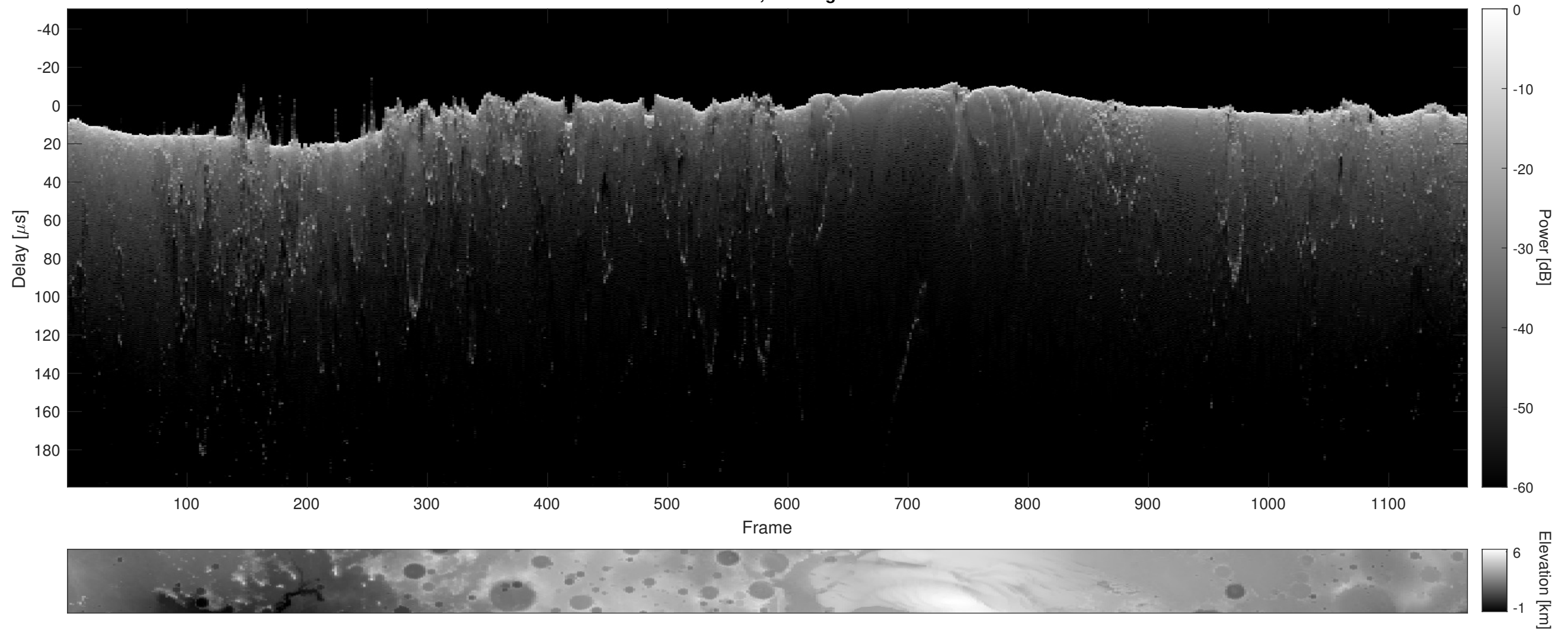
Orbit 13012, Cluttergram
