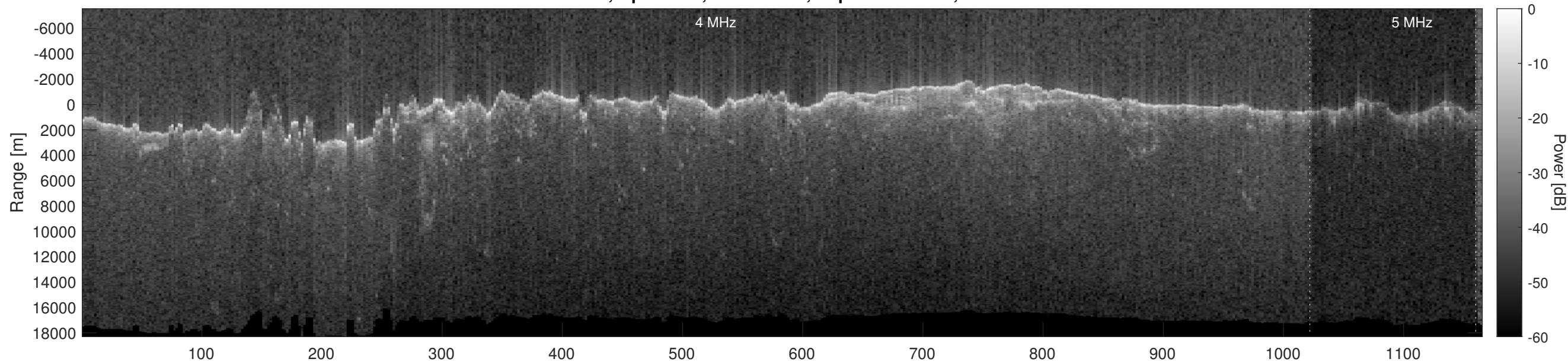
Orbit 13012, Optimized, No Window, Depth-Corrected, Channel 2
