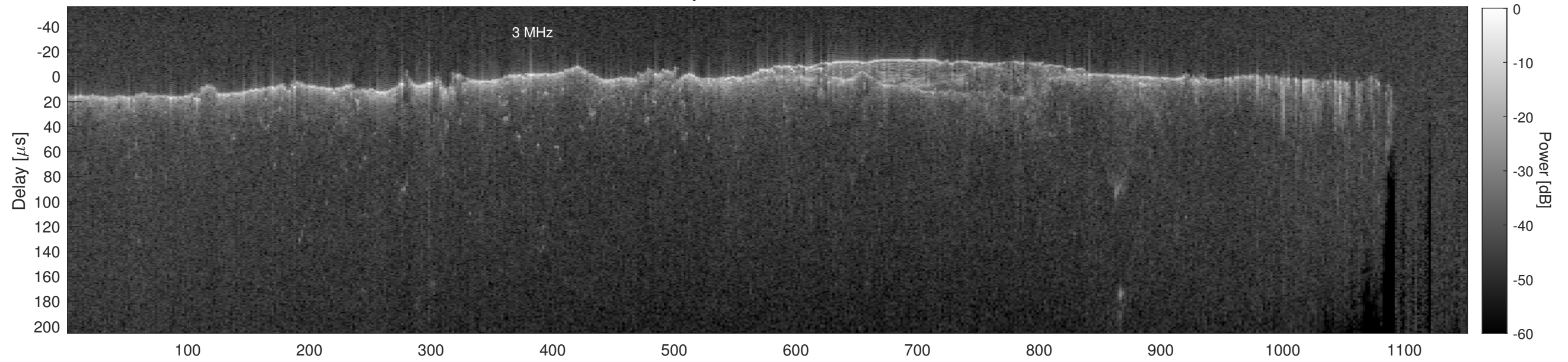
Orbit 13015, Cluttergram
