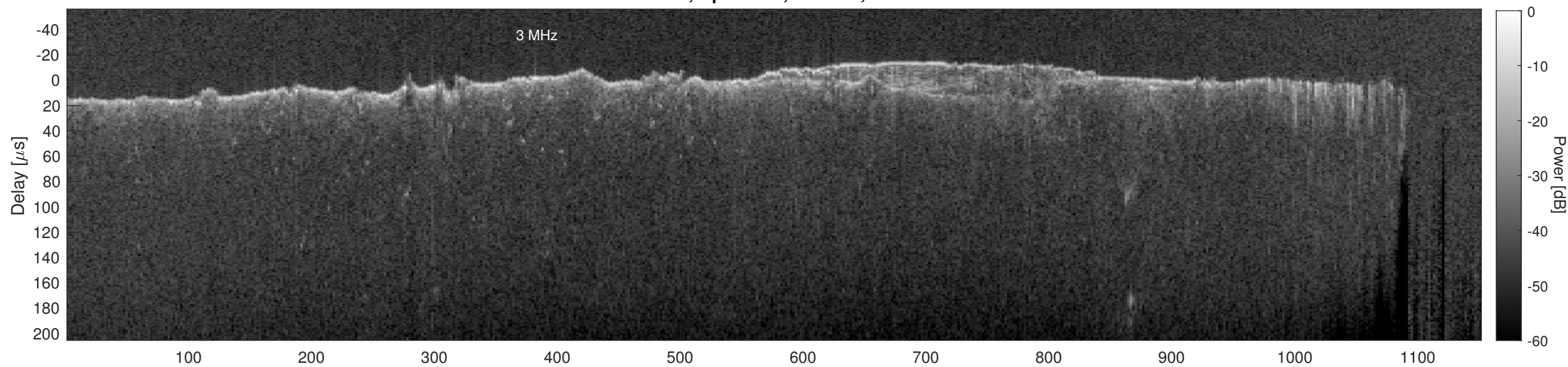
Orbit 13015, Cluttergram
