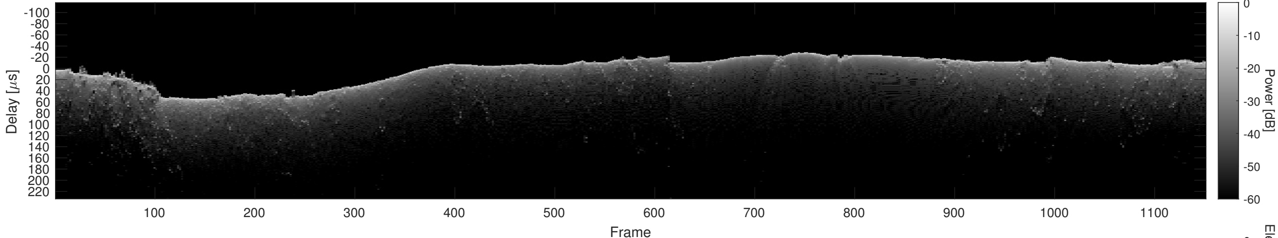
Orbit 13016, Cluttergram
