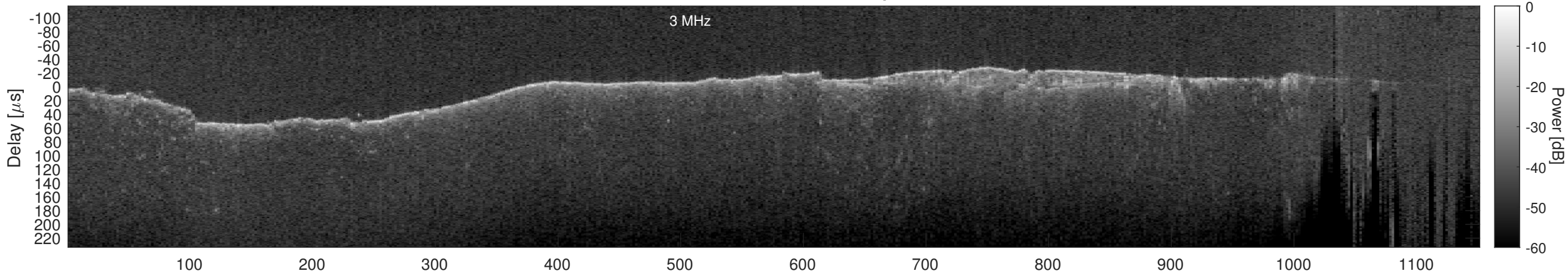
Orbit 13016, Cluttergram
