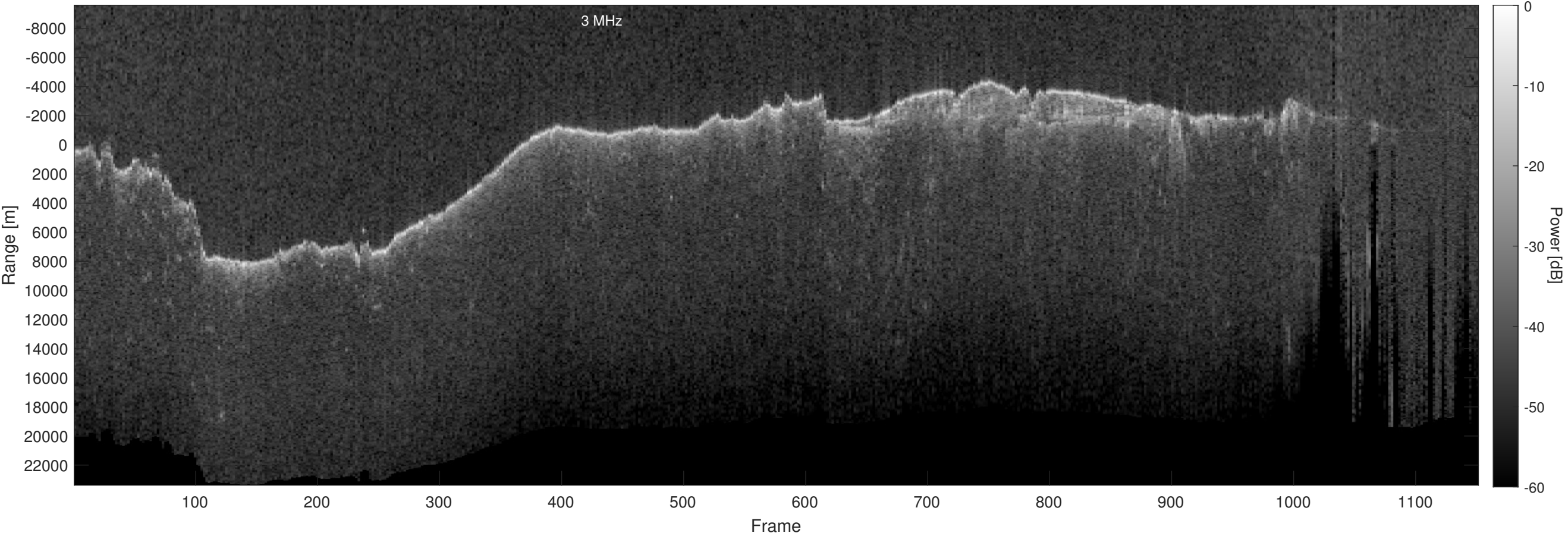
Orbit 13016, Optimized, Window, Depth-Corrected, Channel 2
