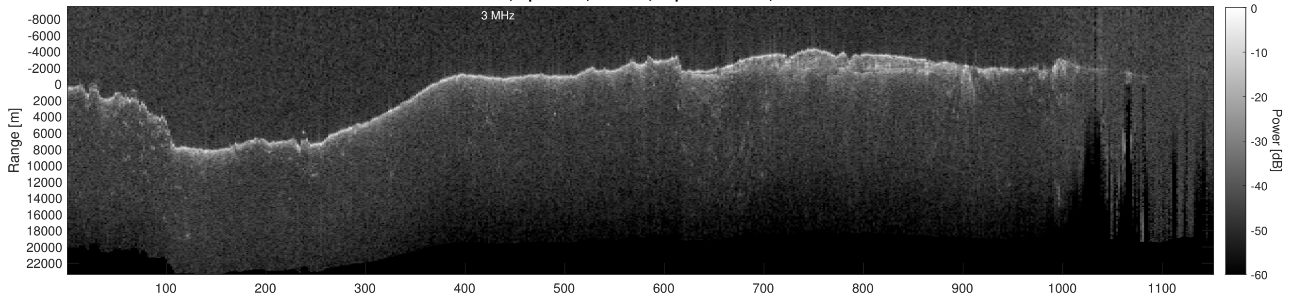
Orbit 13016, Depth-Corrected Cluttergram
