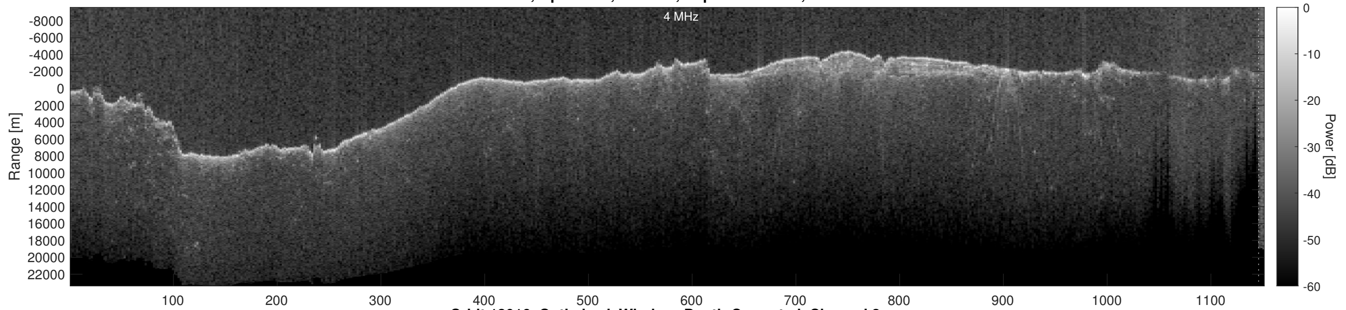
Orbit 13016, Optimized, Window, Depth-Corrected, Channel 2
