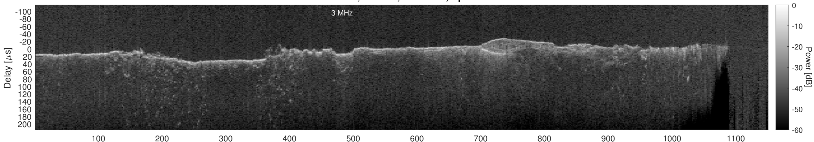
Orbit 13017, Cluttergram
