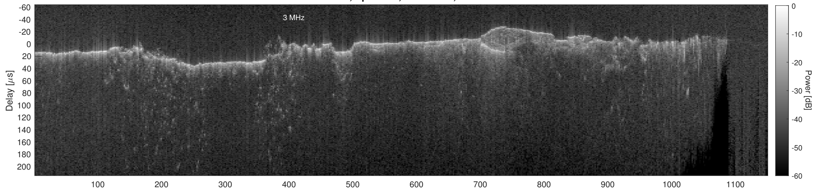
Orbit 13017, Cluttergram
