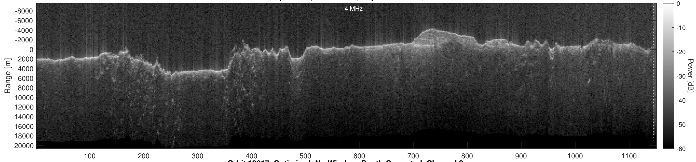
Orbit 13017, Optimized, No Window, Depth-Corrected, Channel 2
